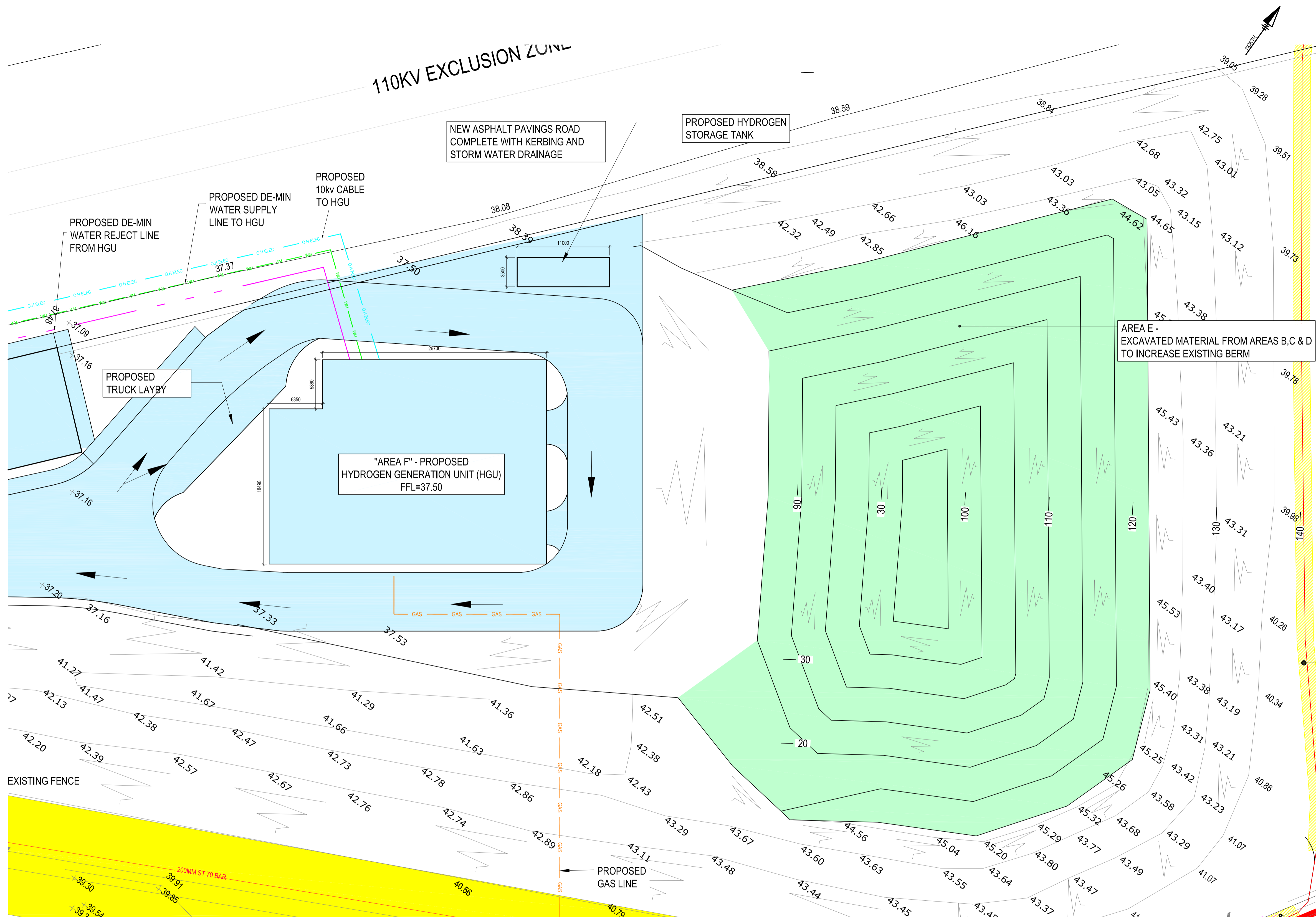
PROPOSED PART SITE PLAN 6 SCALE 1:250
